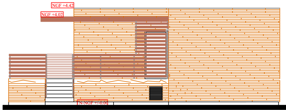
FACADE SUD
